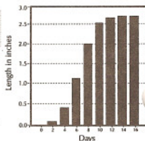
Figure 4. Elongation pattern for internode #14 of an early-maturing variety (Source: J.A. Landivar)
